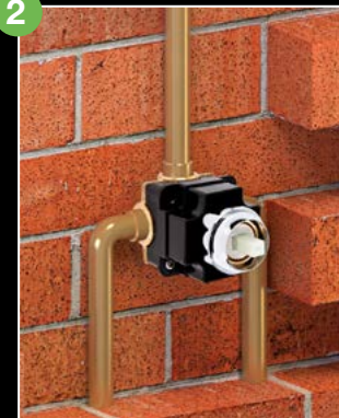
Installation of piping to the concealed part.
